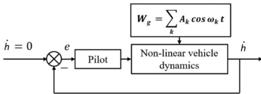
Fig. 6. Pilot-aircraft system in an acceleration task.
