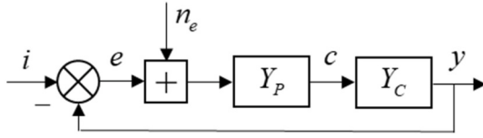
Fig. 4. Compensatory pilot-vehicle system.
