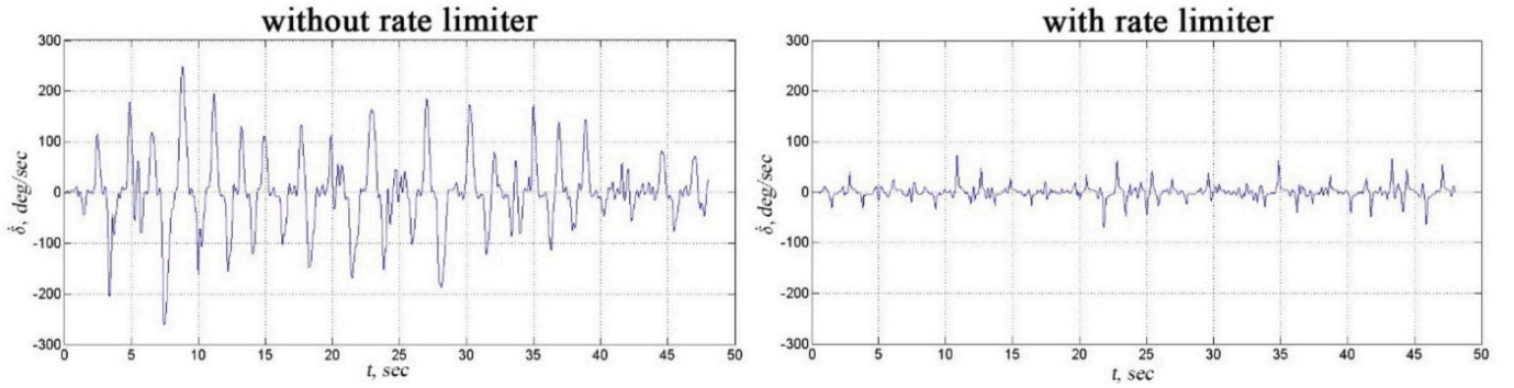
Fig. 18. Required rates of the actuator.
