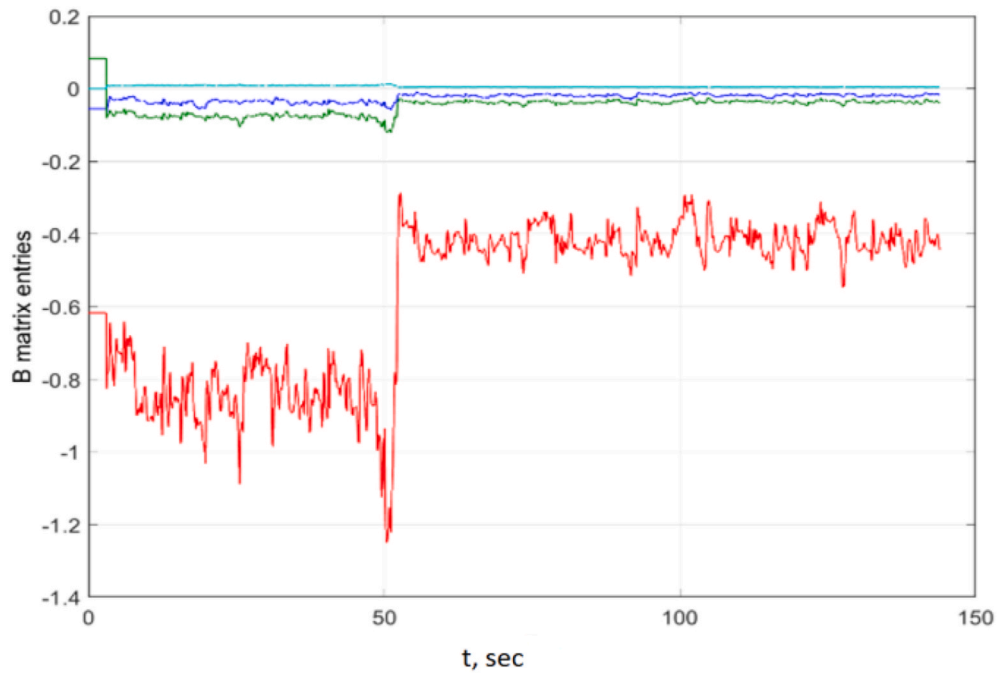
Fig. 11. Adaptation of the coefficients of matrix B.
