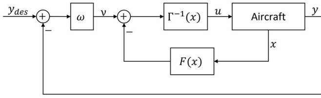
Fig. 1. Schematic of nonlinear dynamic inversion control.
