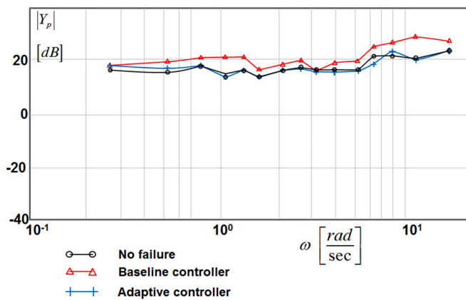
Fig. 12. Pilot frequency response.
