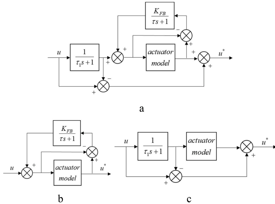
Fig. 16. Rate limiter with feedback and bypass prefilter and its subsystems.
