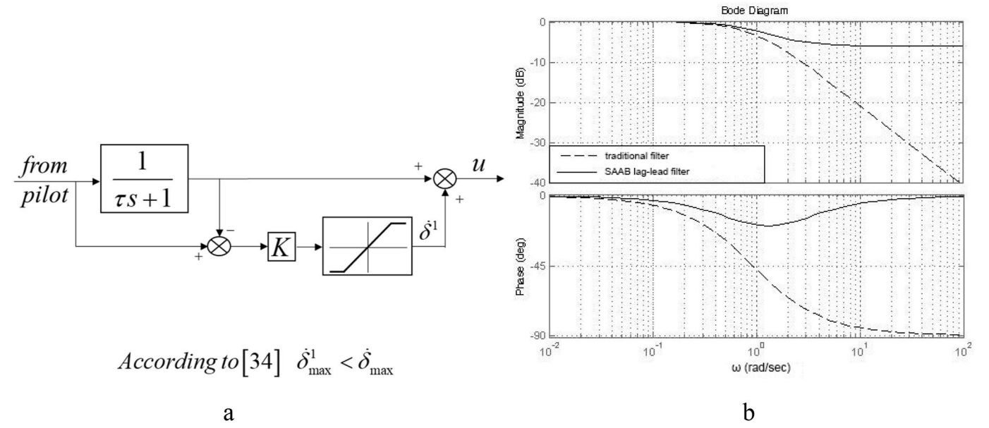
Fig. 15. SAAB nonlinear lead-lag filter (a) and its frequency response (b).
