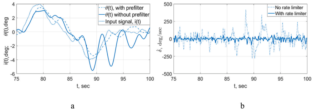
Fig. 19. PIOs in the Space Shuttle experiment (a); the required rates of the actuator (b).
