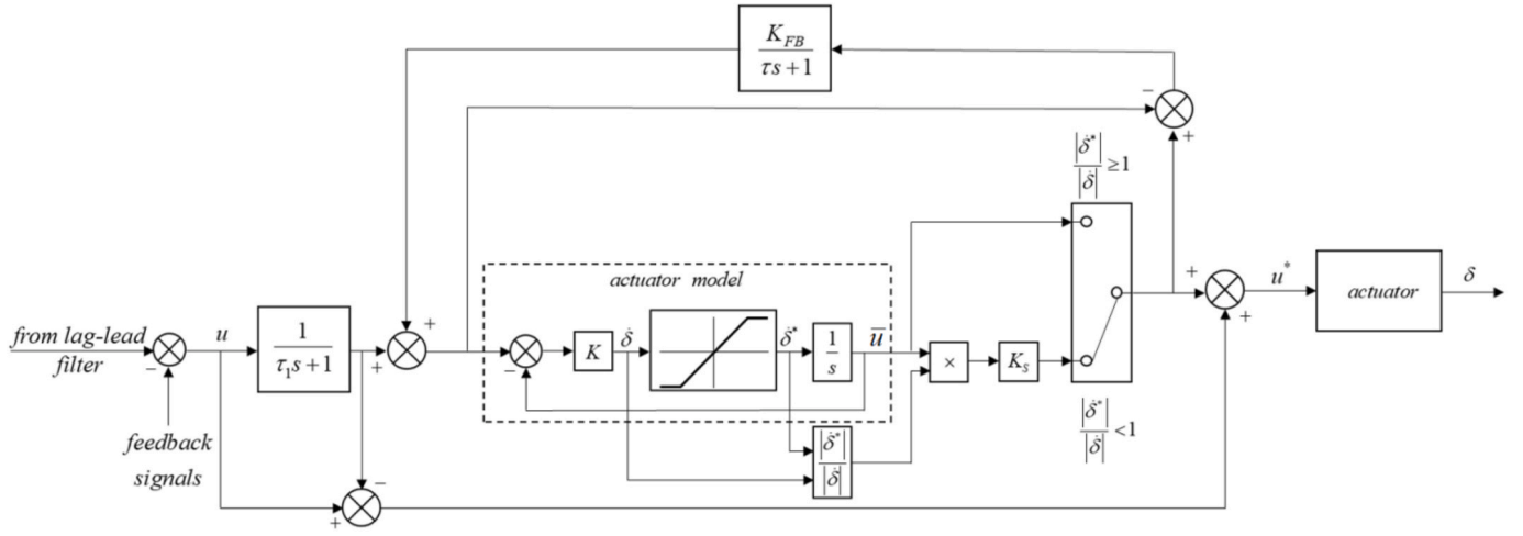
Fig. 17. Modified nonlinear rate limiter with feedback and bypass.
