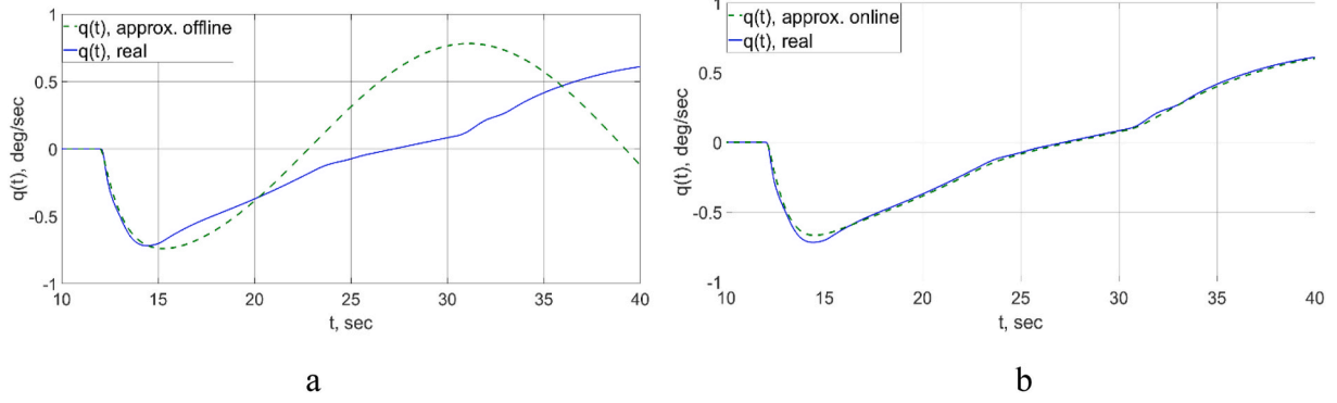
Fig. 3. Comparison of the time responses q(t) obtained by only initial offline identification (a) and online identification (b) with the response q(t) obtained with the real nonlinear model.
