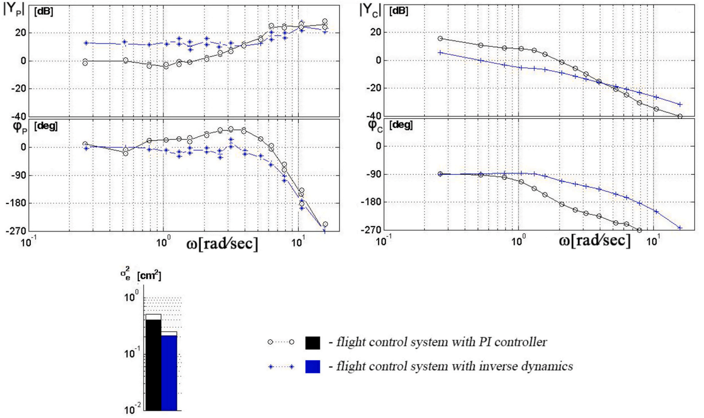
Fig. 8. Experiments on the Space Shuttle dynamics.
